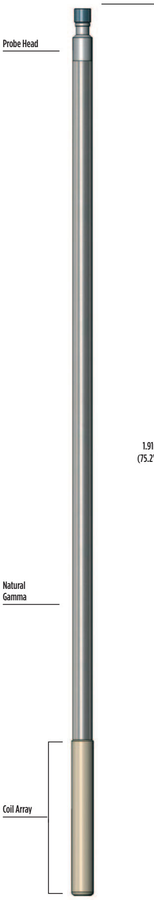
Magnetic Susceptibility Probe
